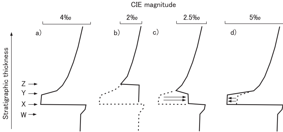
Fig. 2. Schematic diagram explaining artificial alteration of \delta^{13}\text{C} stratigraphy. (a) Assumed pattern for complete record of \delta^{13}\text{C} fluctuation in ocean-atmospheric \text{CO}_2 reservoir without any superimposed signals or stratigraphic missing. (b) Supposed \delta^{13}\text{C} stratigraphy by bulk carbonate analysis with stratigraphic missing between horizons W and Z. Deep sea sediments could lose records of just before the onset and earliest phase of PETM because of “burn down” (see text). Carbonates of horizon W are overlain by that of horizon Z. Note that it appears to be continuous with a conspicuous \delta^{13}\text{C} excursion, in spite of considerable stratigraphic missing. (c) \delta^{13}\text{C} stratigraphy supposed for sedimentary sequence recording oceanographic perturbation just after the onset of PETM; predominance of surface-dwelling nanoplankton associated with shrunk thermocline-dwellers would cause artificial overprint (positive shift) between horizons X and Y. Broken line indicates pattern assumed for record without change of nanoplankton assemblage. (d) \delta^{13}\text{C} stratigraphy supposed for sedimentary sequence recording paleoclimatic perturbation on land between X and Y; predominance of angiosperm overturned from mixed flora of angiosperm and gymnosperm associated with climatic warming, or physiological response of terrestrial plants to increasing temperature and/or humidity would overprint \delta^{13}\text{C} signals on terrestrial biomarkers resulting in an additional negative \delta^{13}\text{C} shift relative to the original (broken line) configuration between X and Y.
